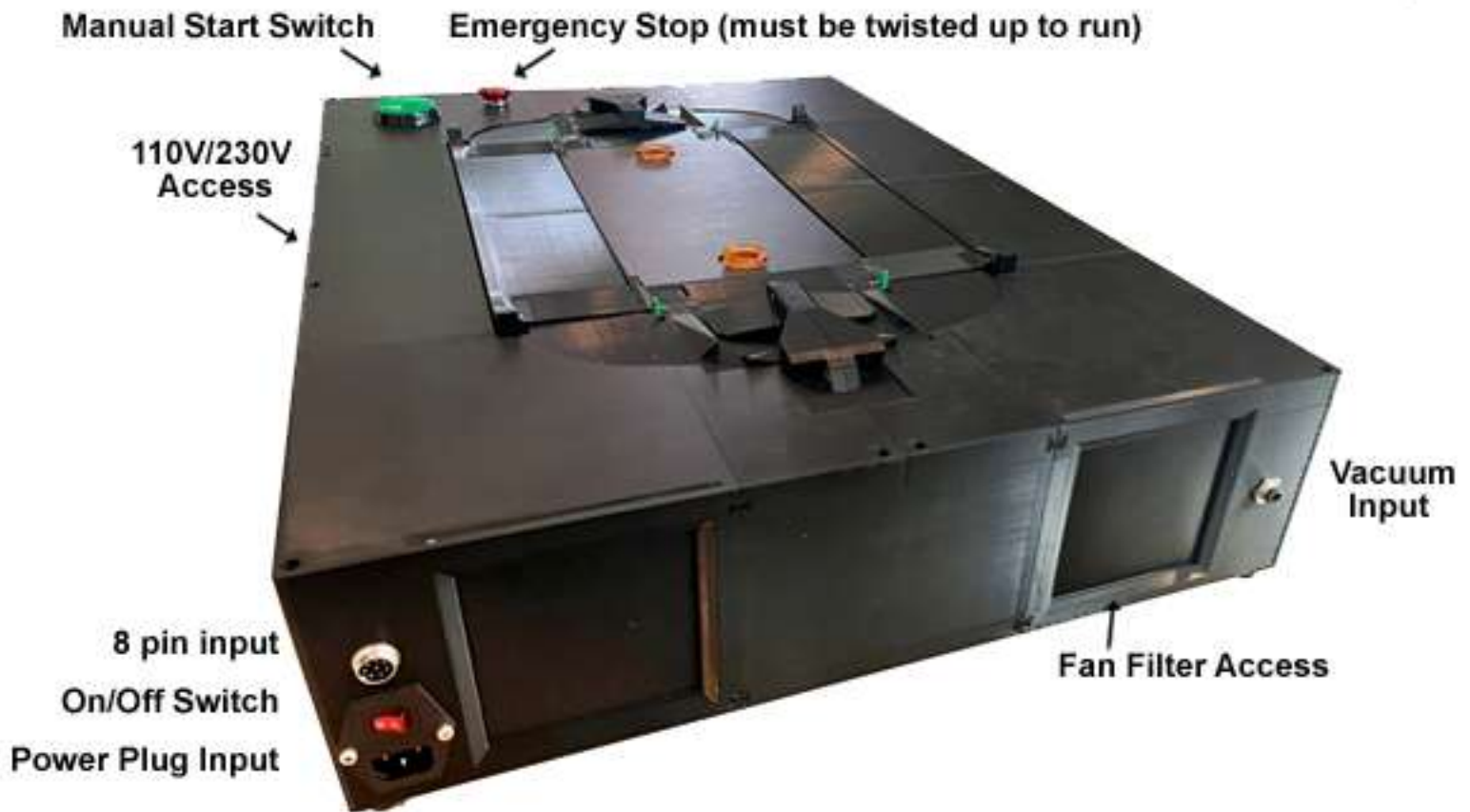
Front Arm
