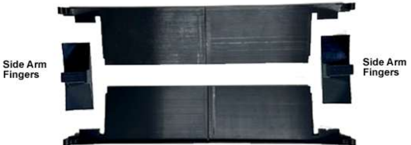
Back Arm
